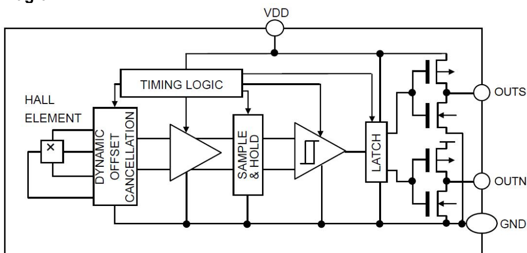
Figure 2, Block Diagram of AS1820A
