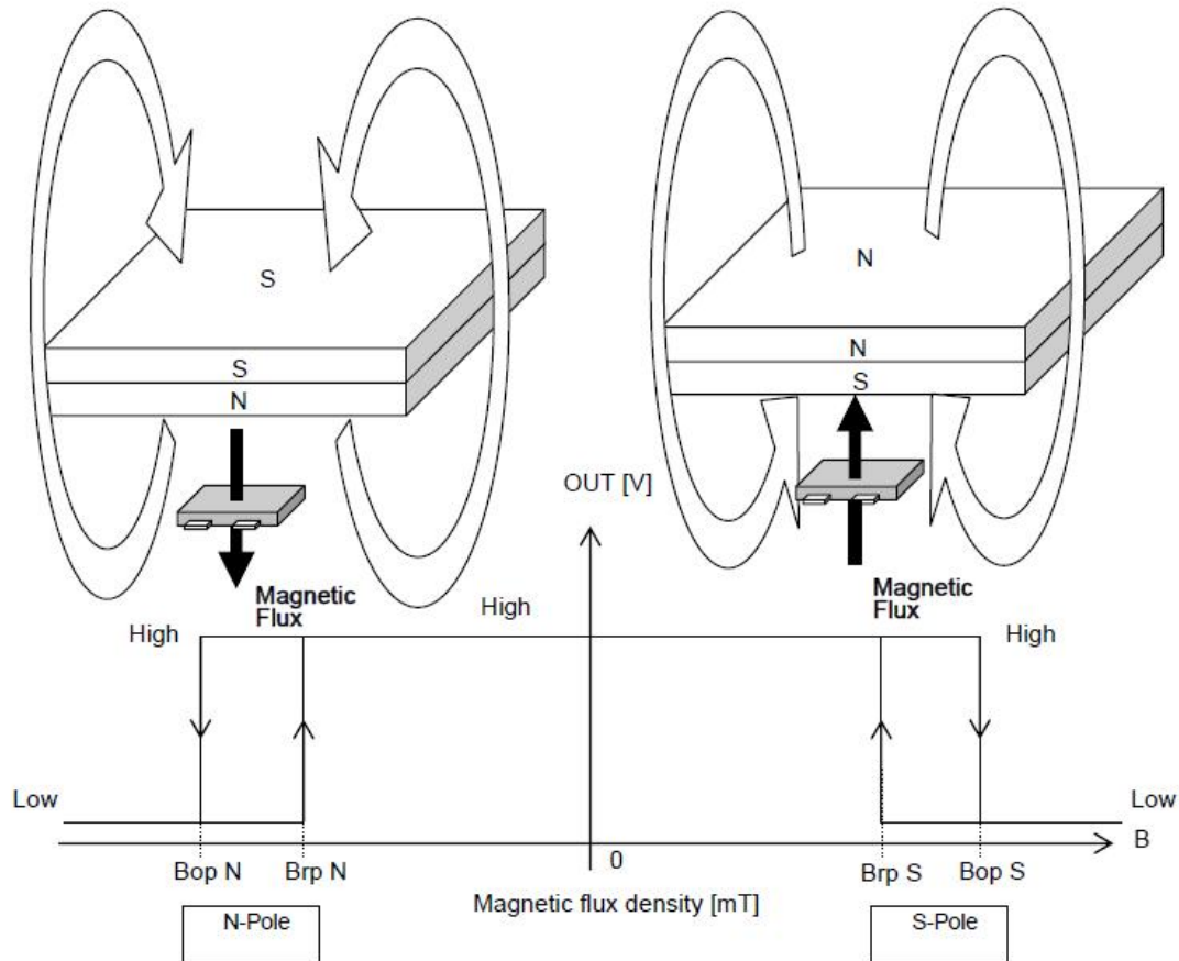
Figure 3, Magnetic Operation Characteristic of AS1820A
